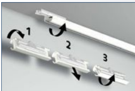
Ceiling click bracket mounting process
