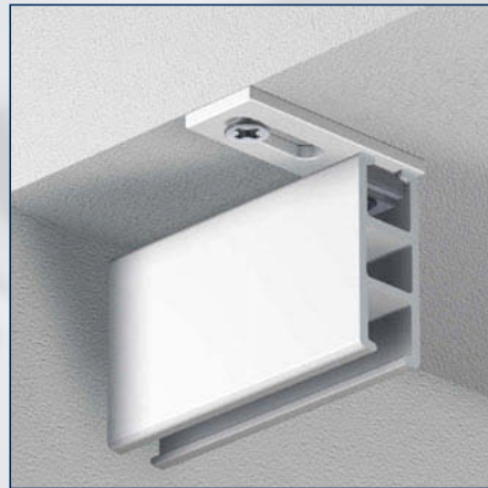
Ceiling bracket with slotted hole
